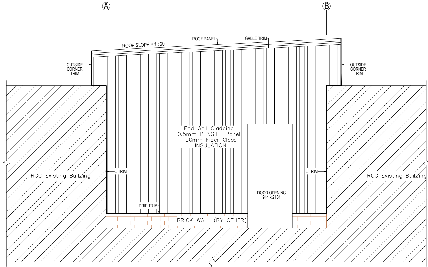
END WALL SHEETING @ GRID-1
